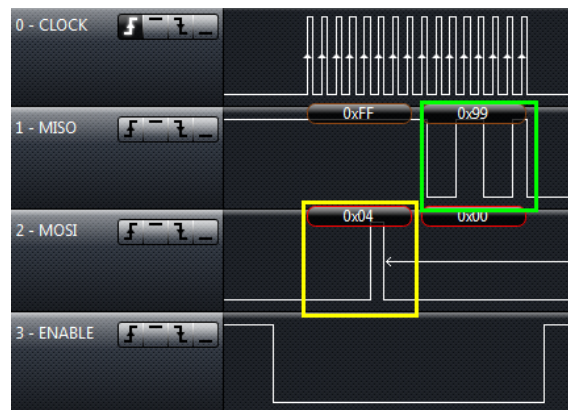
Figure 4-7. Waveform Graph 3
