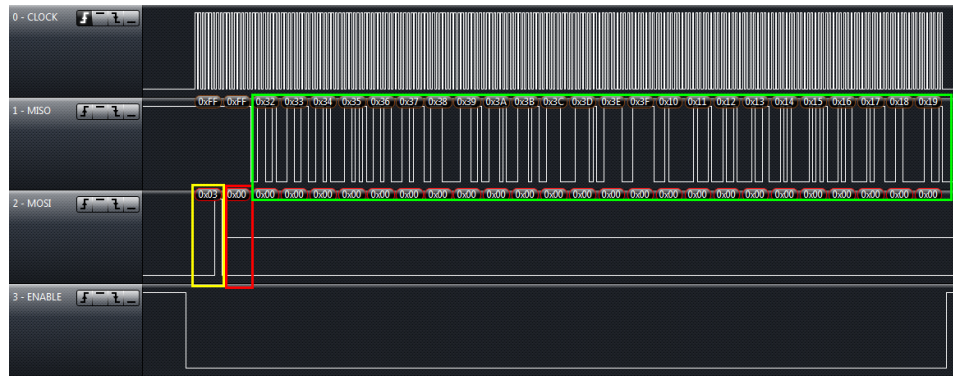
Figure 4-6. Waveform Graph 2
