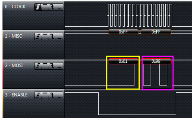
Figure 4-8. Waveform Graph 4
