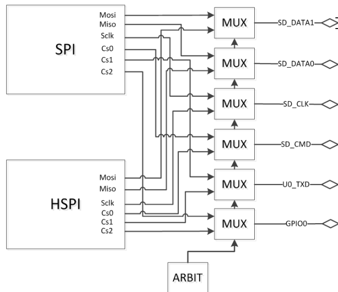
Figure 5-1. SPI Overlap Block Diagram
